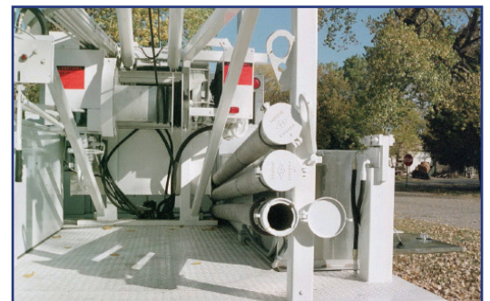
Self contained pump/development rig features an on-board steam cleaner and discharge pipe decontamination tubes
